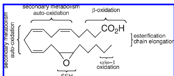
Figure 1. Metabolism/Degradation of 14,15-EET.
