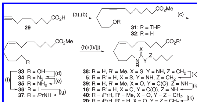
Scheme 1. Synthesis of Representative Analogues a
